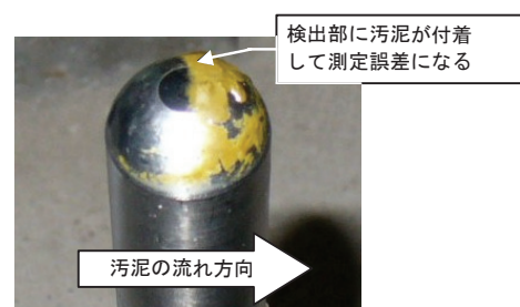
Fig.9: Situation of The Adhesion of Sludge to The Detector
