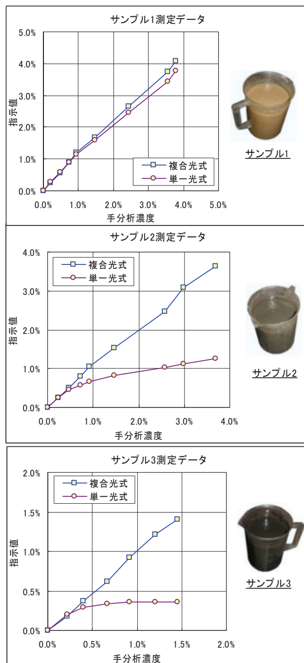
Fig.5: Performance Comparison of Sludge Density Meter
