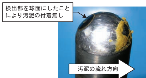
Fig.13: After Revised The Structure of The Detector
