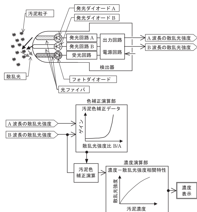
Fig.4: Measurement Principle of Optical Density Meter (Dual Light)
